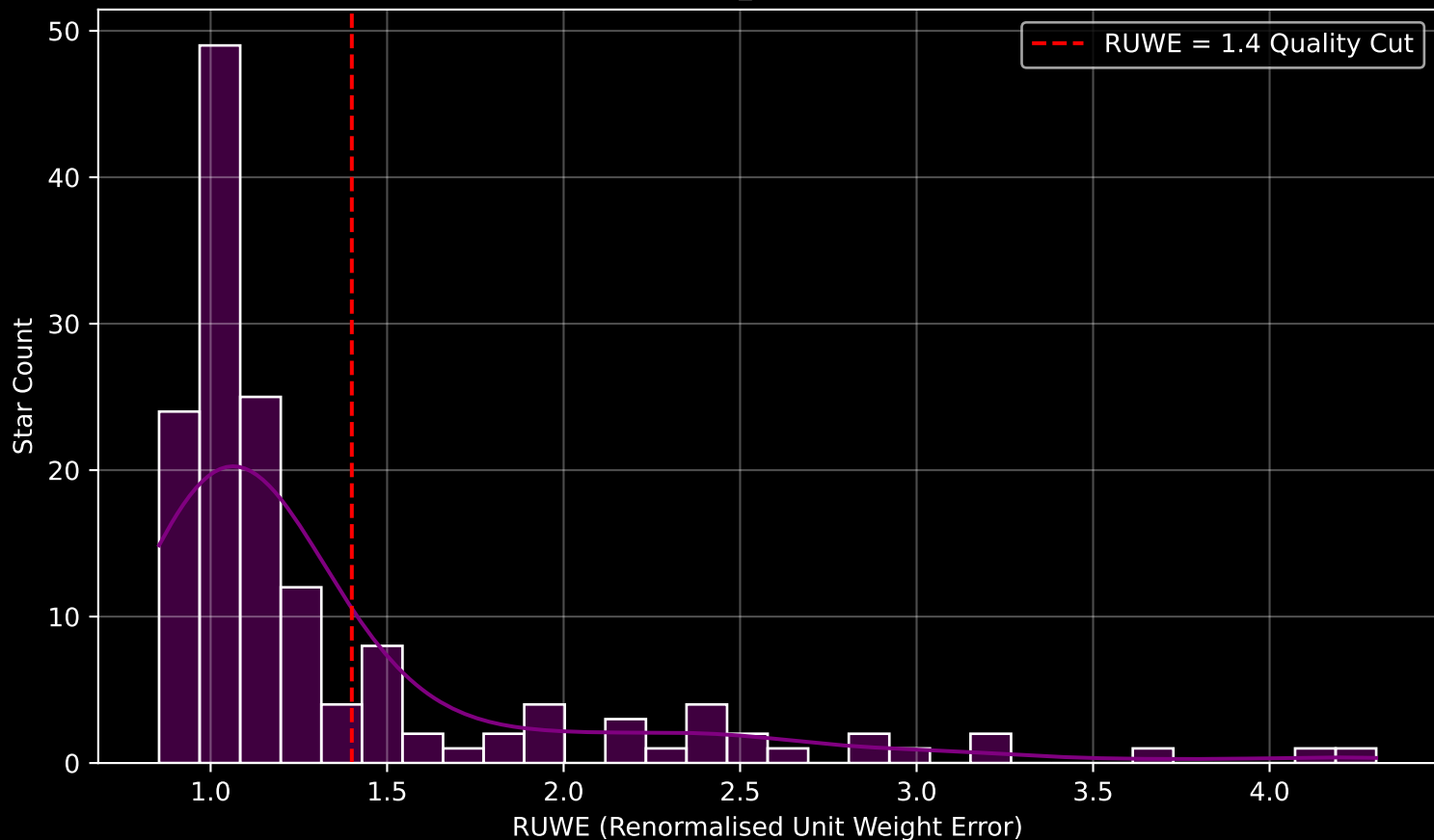
GAPOGEE DR17 Field [039+46_MGA] RUWE Distribution (n= 150)
