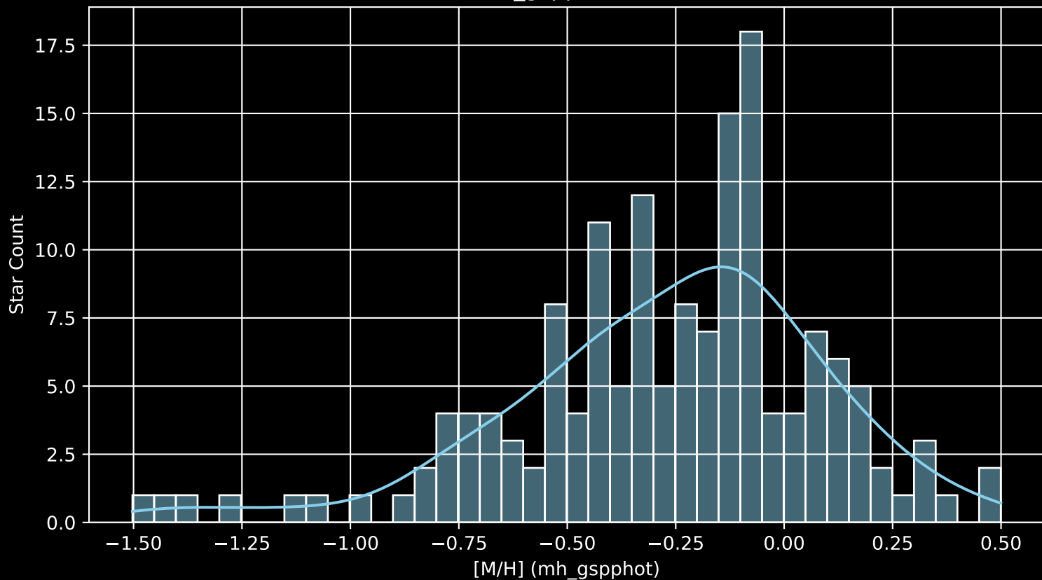
APOGEE DR17 Field: [039+46_MGA [M/H] (mh_gspphot) (n= 155)
