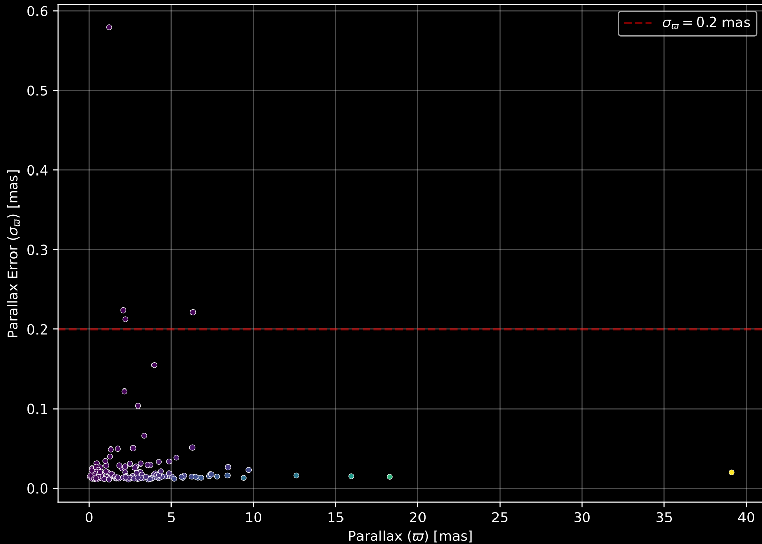
APOGEE DR17 Field: [039+46_MGA] Parallax Quality (n= 157)
