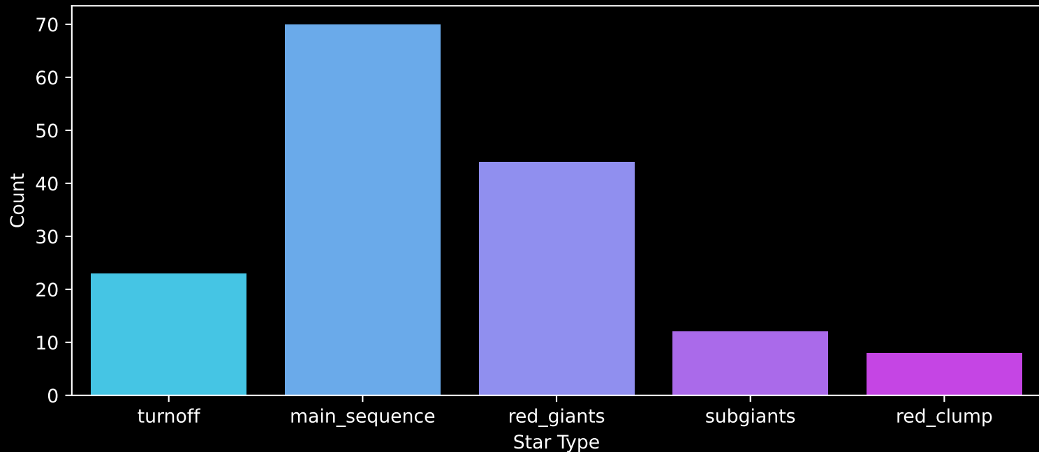
APOGEE DR17 Field: [039+46_MGA] Count plot of Star Type
