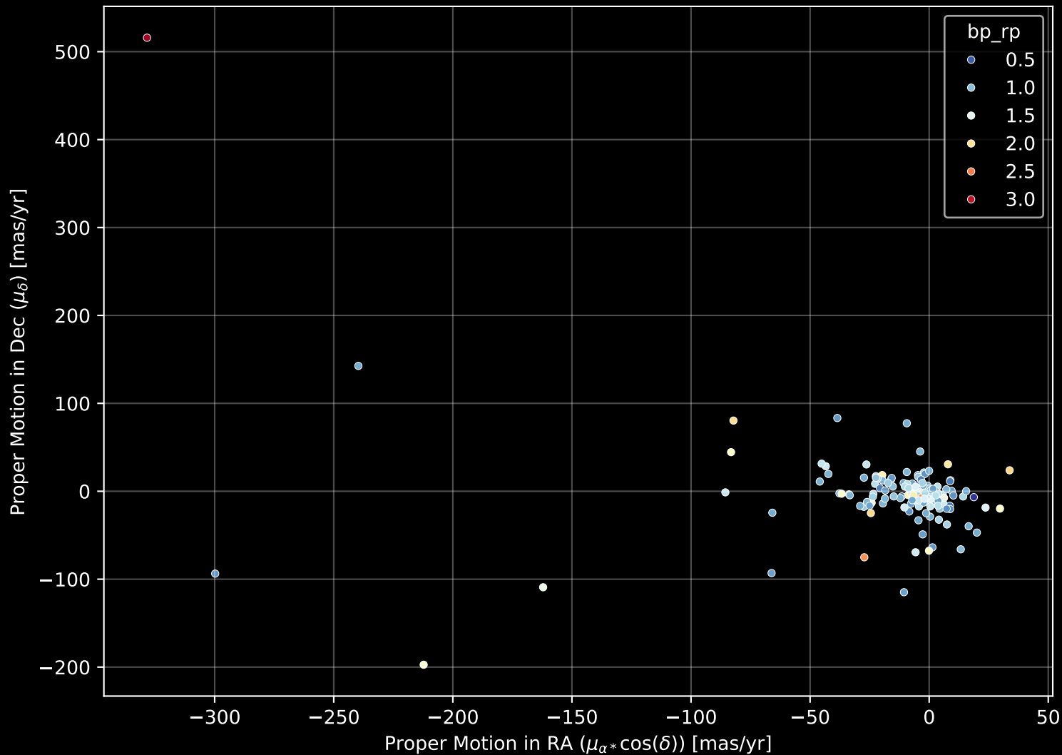
APOGEE DR17 Field: [039+46_MGA] Proper Motion Diagram (n= 157)
