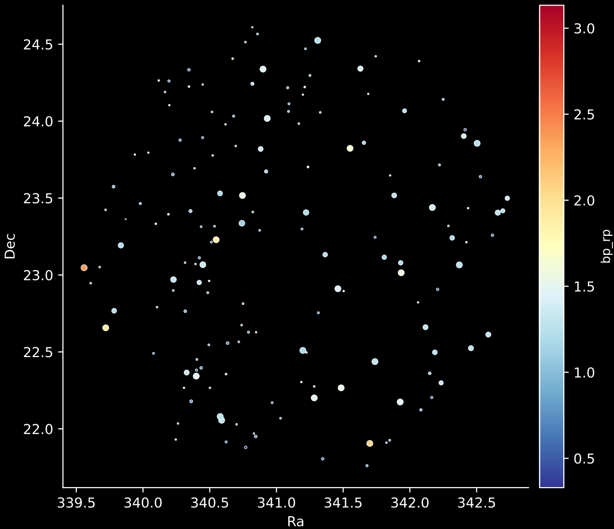
APOGEE DR17 Field: [039+46_MGA] Stars: 157
